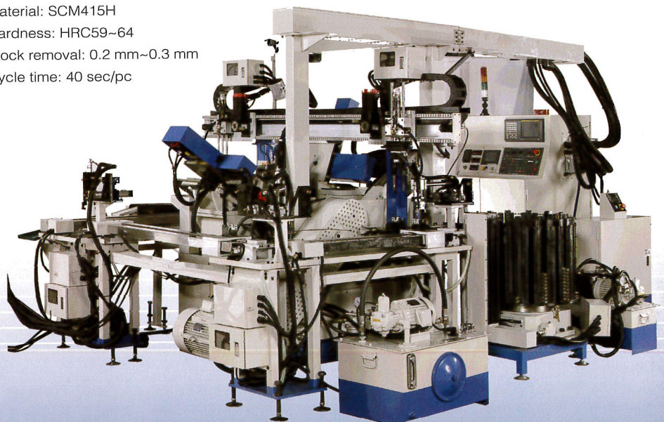
JHC-18 CNC 8 axes with robot system and relay transplanter for grinding universal joint kits. (Rotor system is for loading & unloading)
