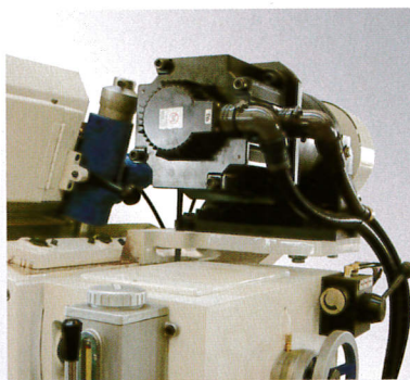
JHC-12S with servo motor for regulating wheel, variable speed.
