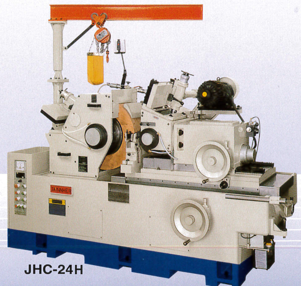
Lower Slide Way is equipped with Heavy Bearing, Linear Motion System and Ball Screws.
