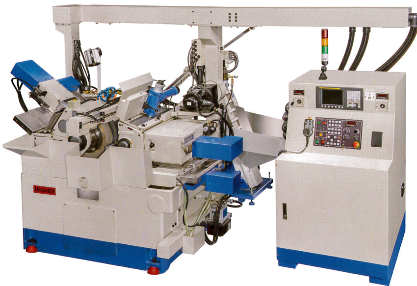
JHC-18S-CNC6 Axes for grinding automobile engine valve
