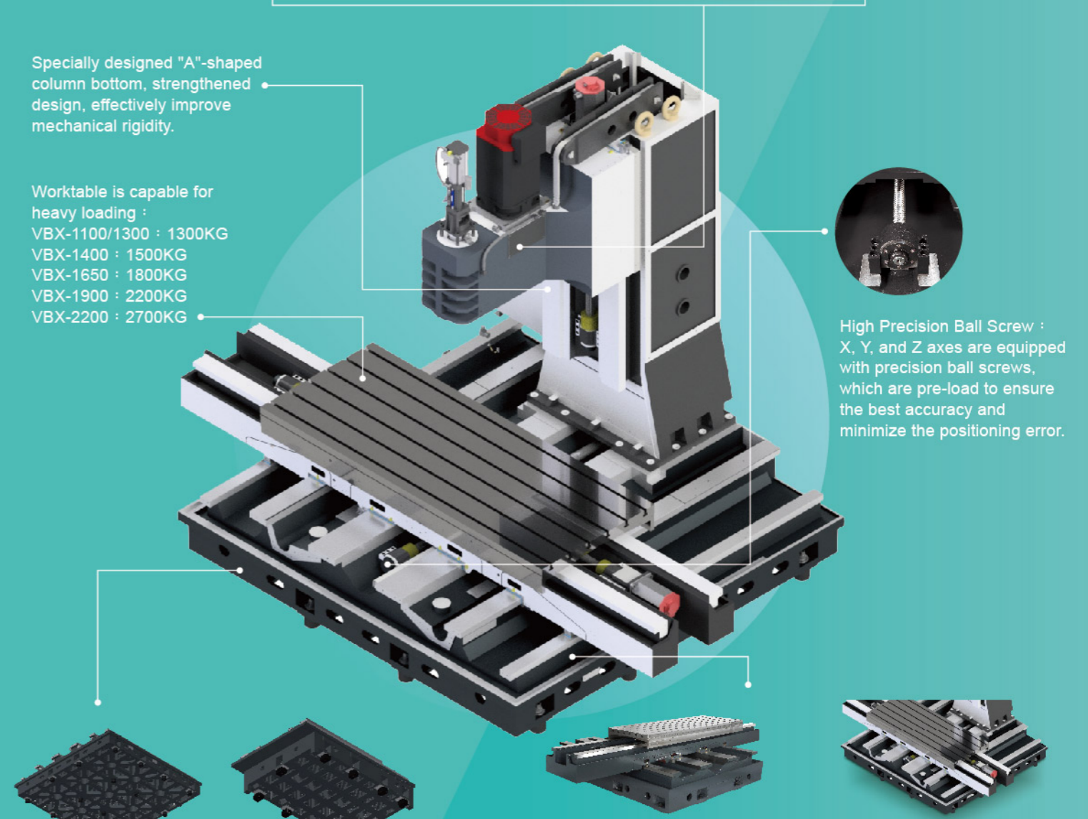
VBX-1100/1300/1400/1650/1900 Four Box Ways Base
